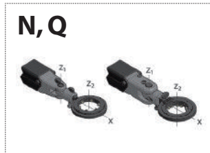
N:from 0 up to 15 kg with Quick change X:Turns 360°. Lockable 4x90°. Z1:Turns 90° right & left. Z2:Turns 360°. Q:from 15 up to 30 kg X:Turns 360°. Lockable in any position Z1:Turns 90° right & left Z2:Turns 360°. Lockable in any position
