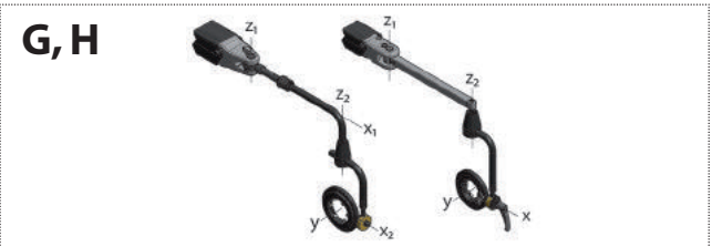
G:from 0 up to 15 kg/33 lbs with Quick Change X1:Turns 360°. Lockable each 45° X2:Turns 360°. Y:Turns 360°. Z1:Turns 90° right & left. Z2:Turns 360°. Non lockable H:from 15 kg/33 lbs up to 30 kg/66 lbs. NO Quick Change X: turns 360°. Lockable in any position Y:Turns 360°. Lockable in any position Z1:Turns 90° right & left Z2:Turns 360°
